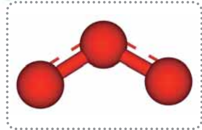
The ozone molecule consists of 3 oxygen atoms. The chemical formula for ozone is O 3 .
